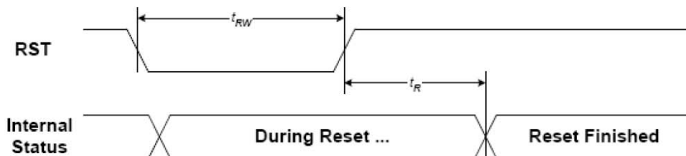
FIGURE 20: Reset Characteristics
