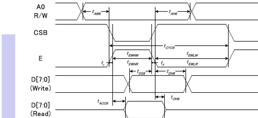
1. 从 CPU 写到 ST75256 (Writing Data from CPU to ST75256)
